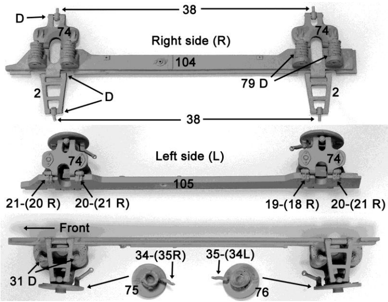
Sub assembly 1 (L + R)
